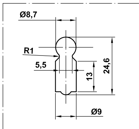
Detalle del agujero Detail of the keyhole
